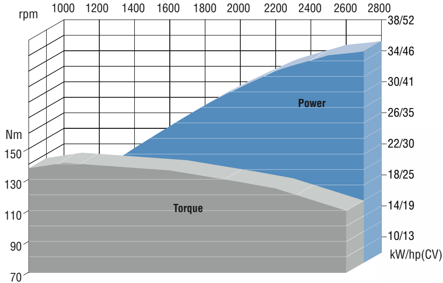
T3030 curves
